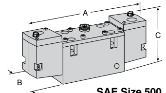
SAE Size 500 Double Solenoid
