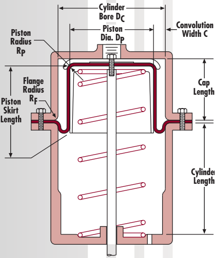
Fig. 17: Hardware Dimensions
