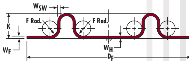
Fig. 10: Preconvoluted Diaphragm
