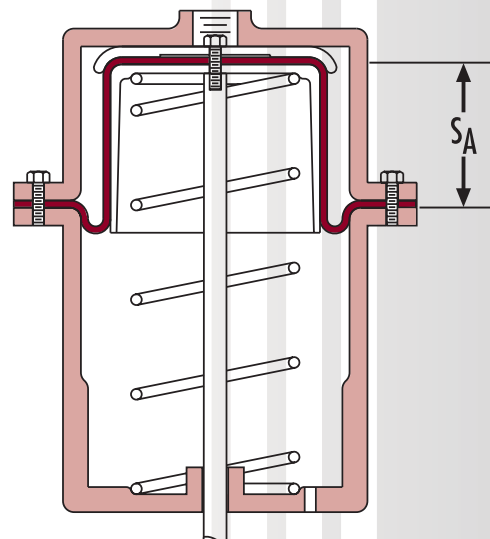
Fig. 7: Up-Stroke Position
